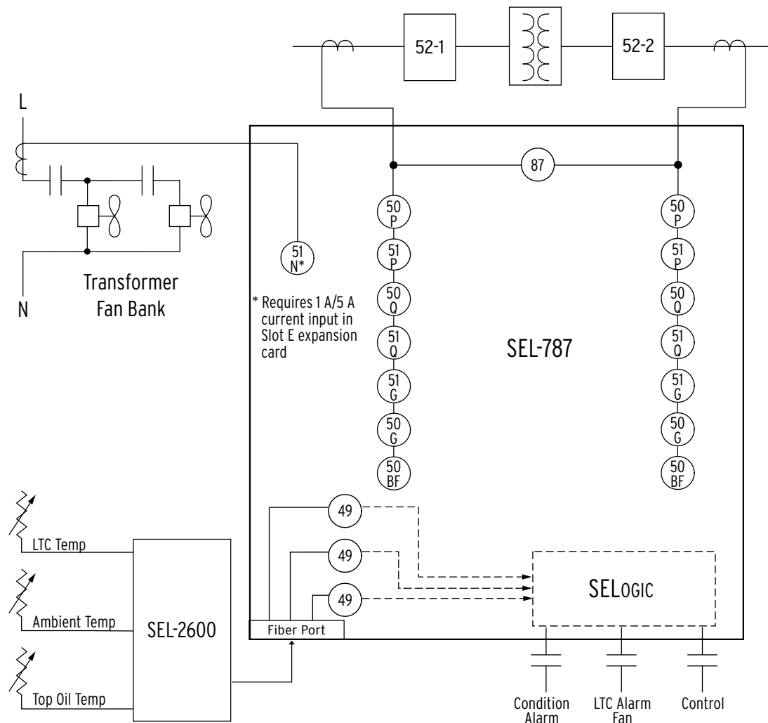
Figure 6 Transformer Fan Bank Control With LTC Monitoring
