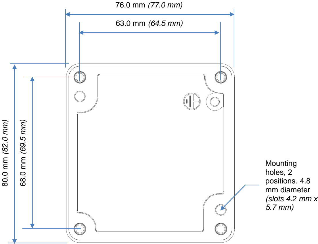
Figure 1 - Dimensional Differences of Terminal Box
