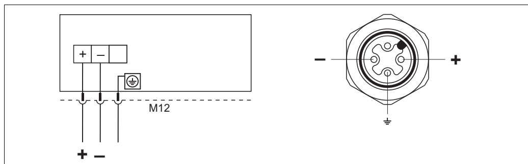
Left: electrical connection for devices with an M12 connector Right: view of the connector at the device
