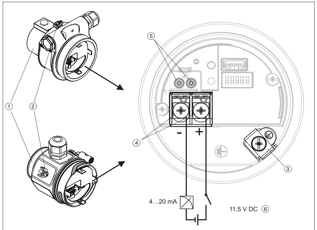
Electrical connection 4 to 20 mA HART
