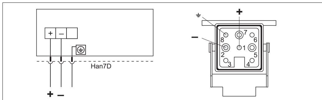
Left: electrical connection for devices with a Harting connector Han7D Right: view of the connection at the device
