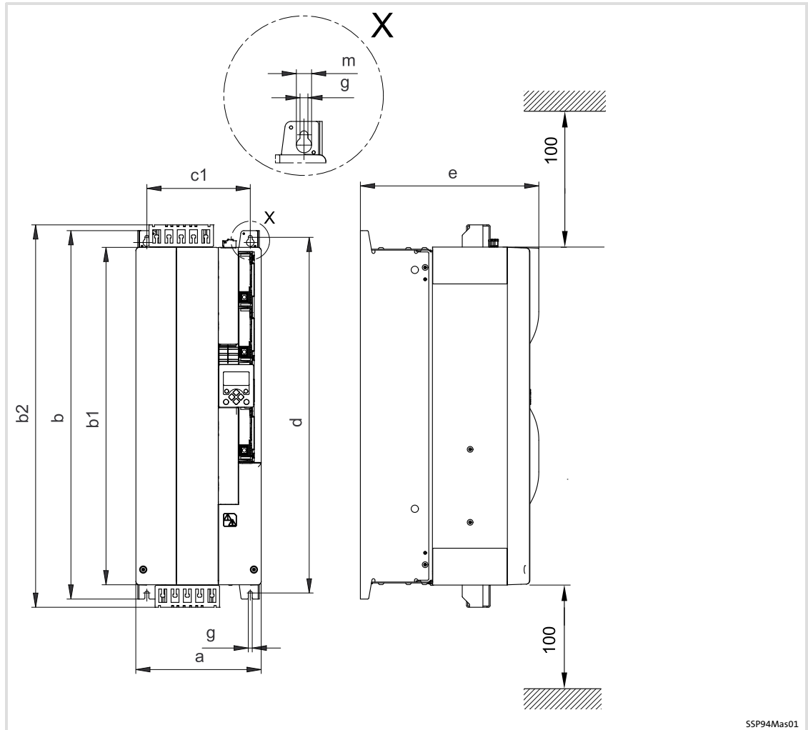
Fig. 3-16 Dimensions [mm]
