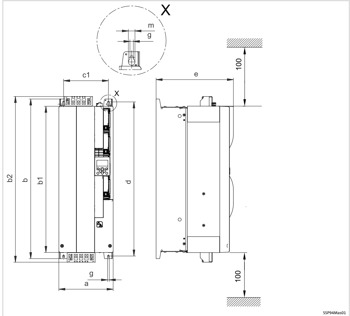
Fig. 3-16 Dimensions [mm]
