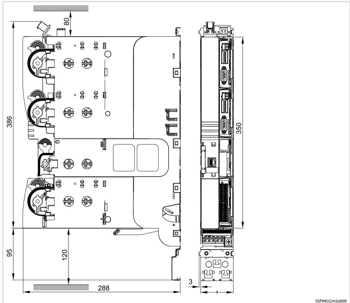
Fig. 3-15 Dimensions [mm]
