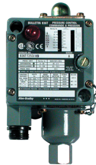
Style T — Type 1, 4 & 13 with Pilot Light, Range Locking Cap, and 5-Pin Mini-Receptacle
