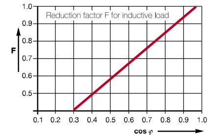
Contact Lifetime
