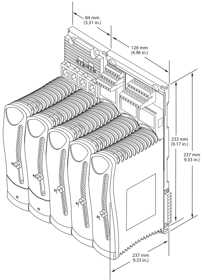
Figure 25 - System Dimensions
